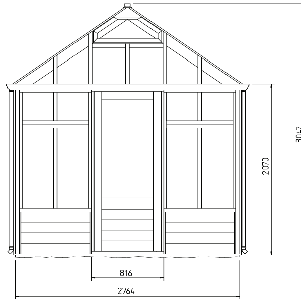
Small Elevation
