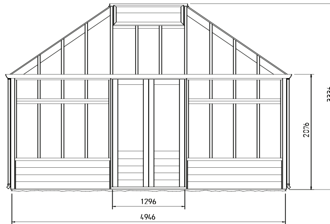
Large Elevation
